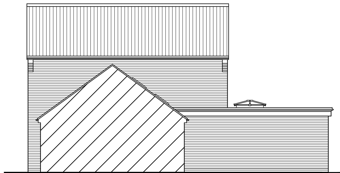
South 6340 Proposed Addition
