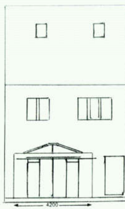
Proposed Rear Elevation 1:100
