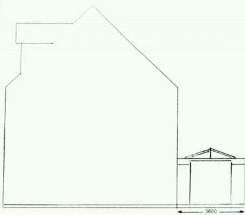
Proposed Left Elevation 1:100
