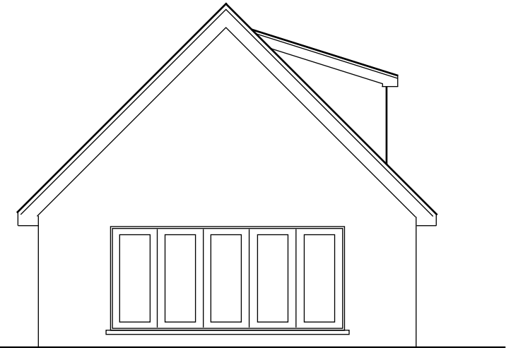
Proposed NE/Rear Elevation
