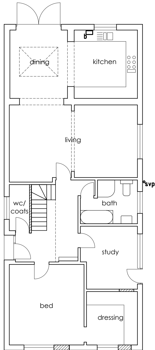
GROUND 1:100
