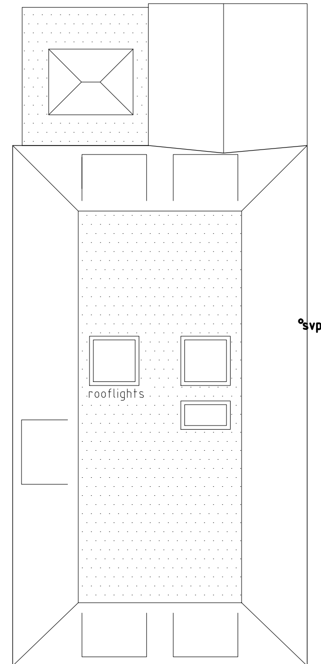
ROOF 1:100
