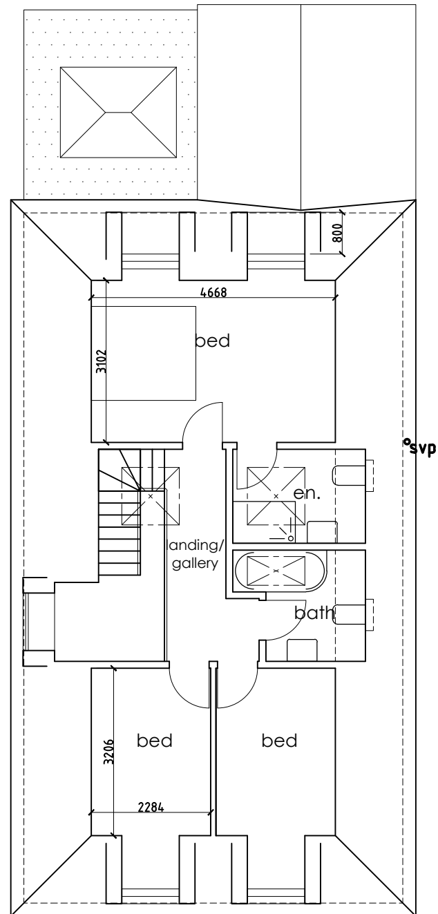
FIRST 1:100
