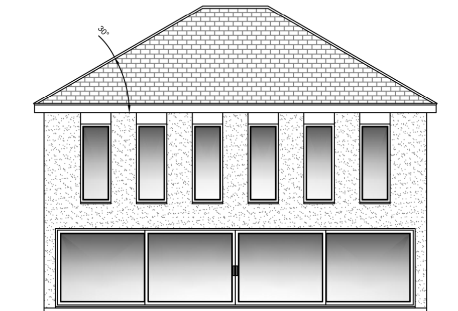
Rear Elevation
