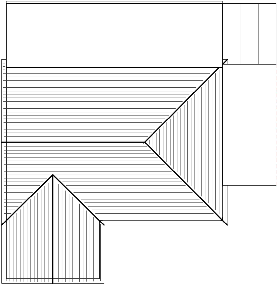
ROOF PLAN
