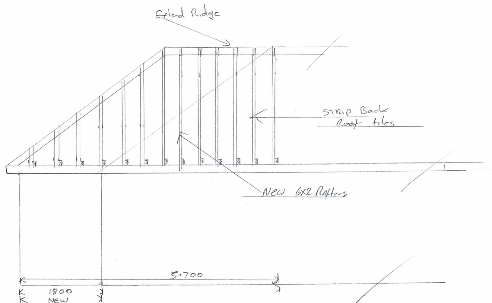
Rear Extension Side Section
