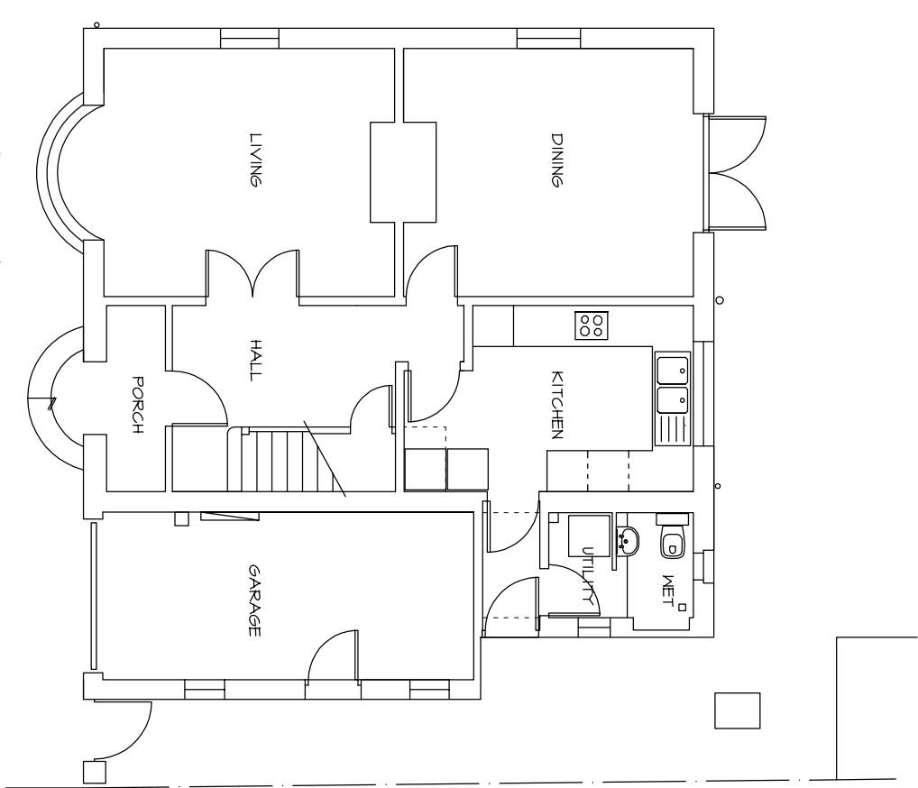
Existing Ground
