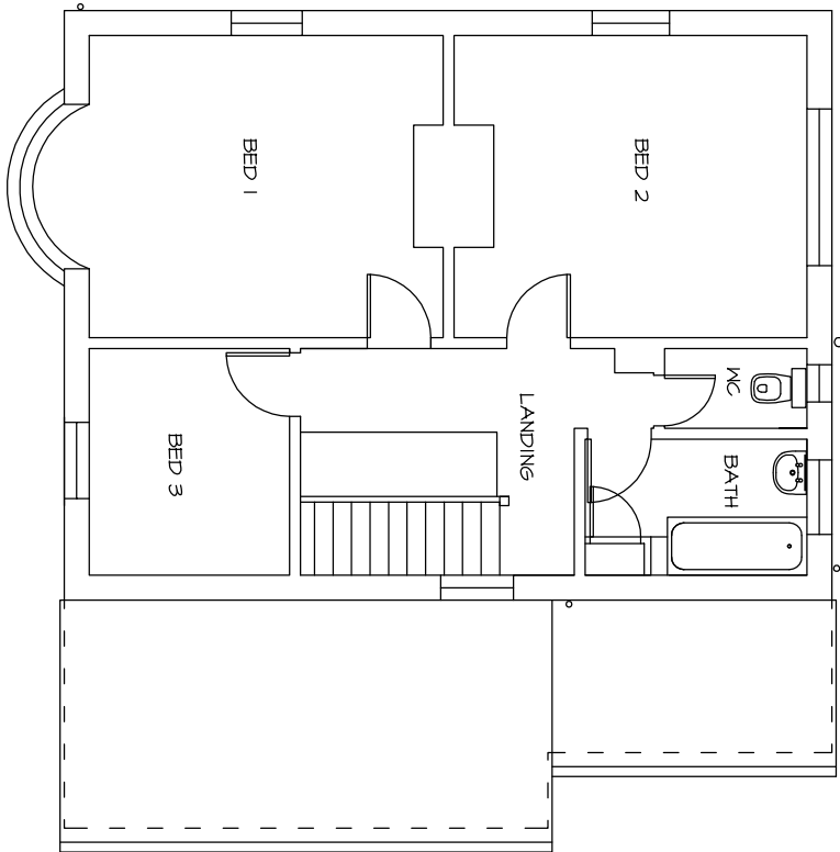
Existing First
