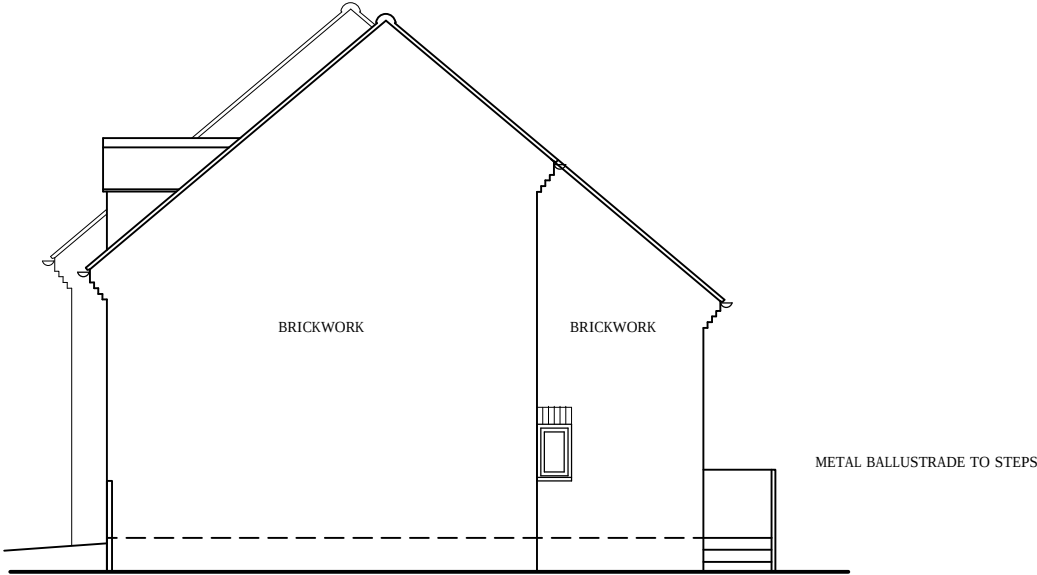
SIDE ELEVATION
