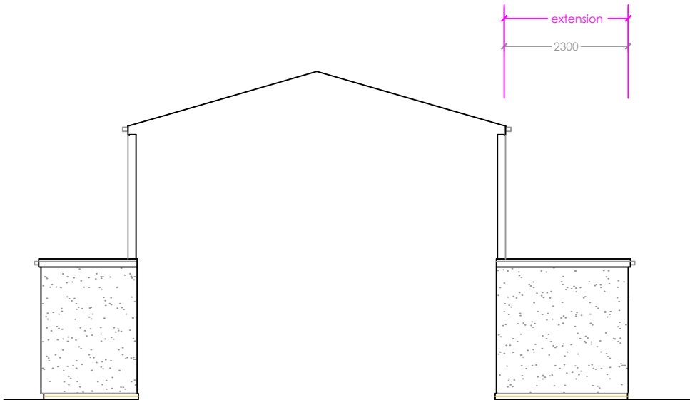
Side Elevation (from no. 28)
