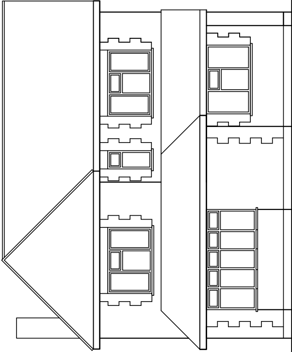
NORTH ELEVATION
