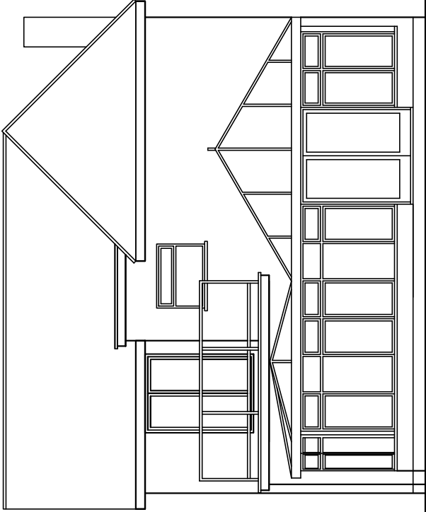
SOUTH ELEVATION
