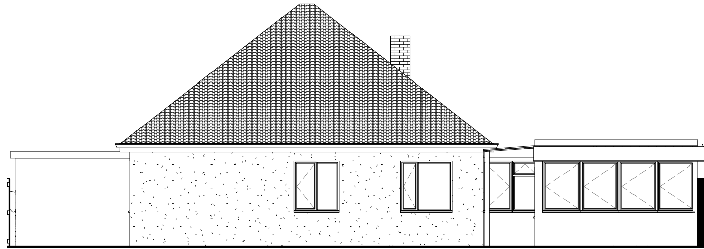
2 North Elevation 1 : 100
