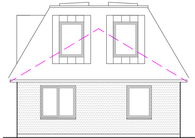
FRONT (N) 1:100
