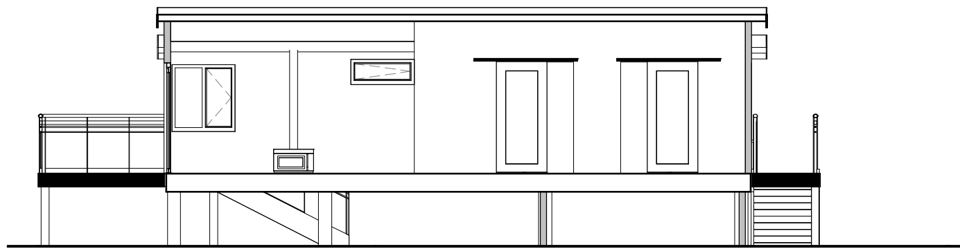
2 North south site section 1 : 100
