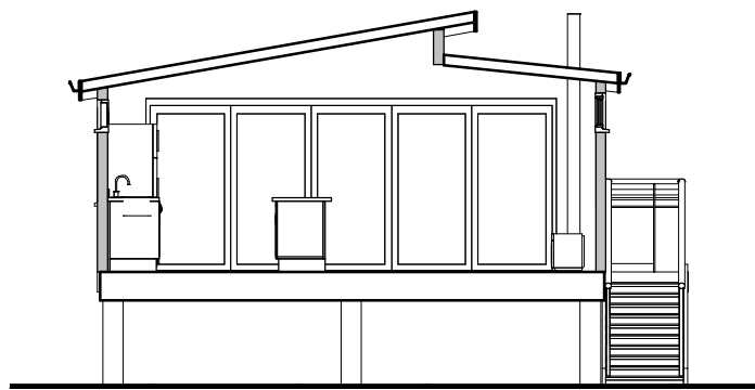
1 East west site section 1 : 100
