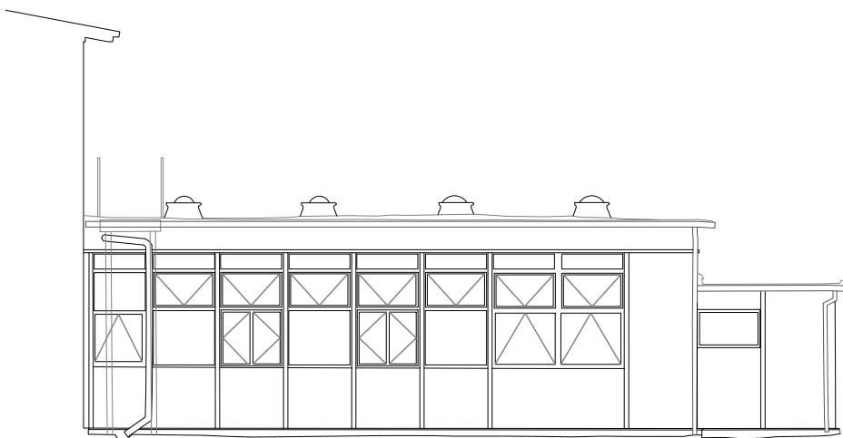
West Elevation - Building Ref 'D' Drg - 315 (2)
