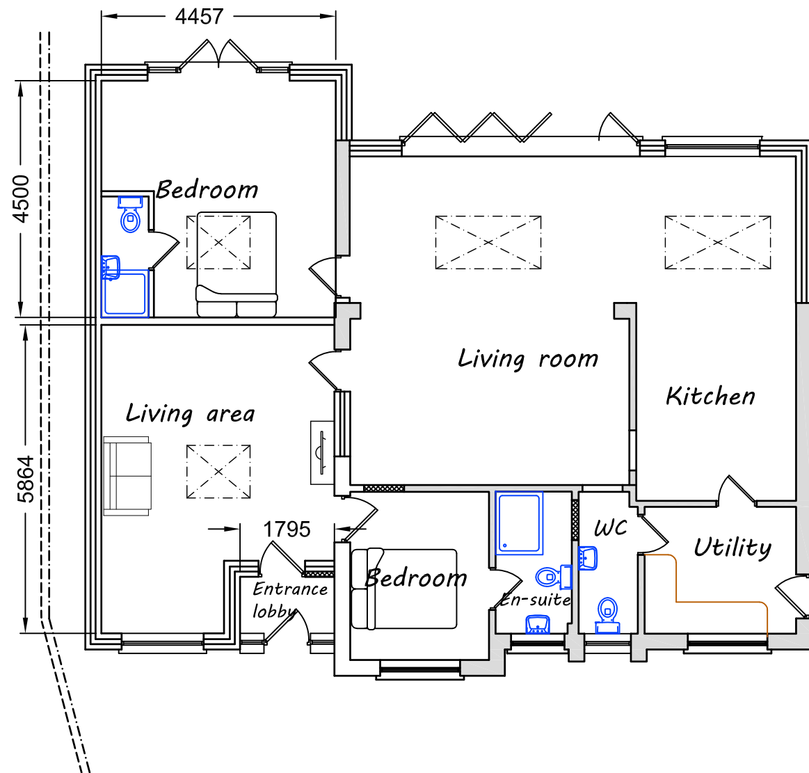
Floor Plan
