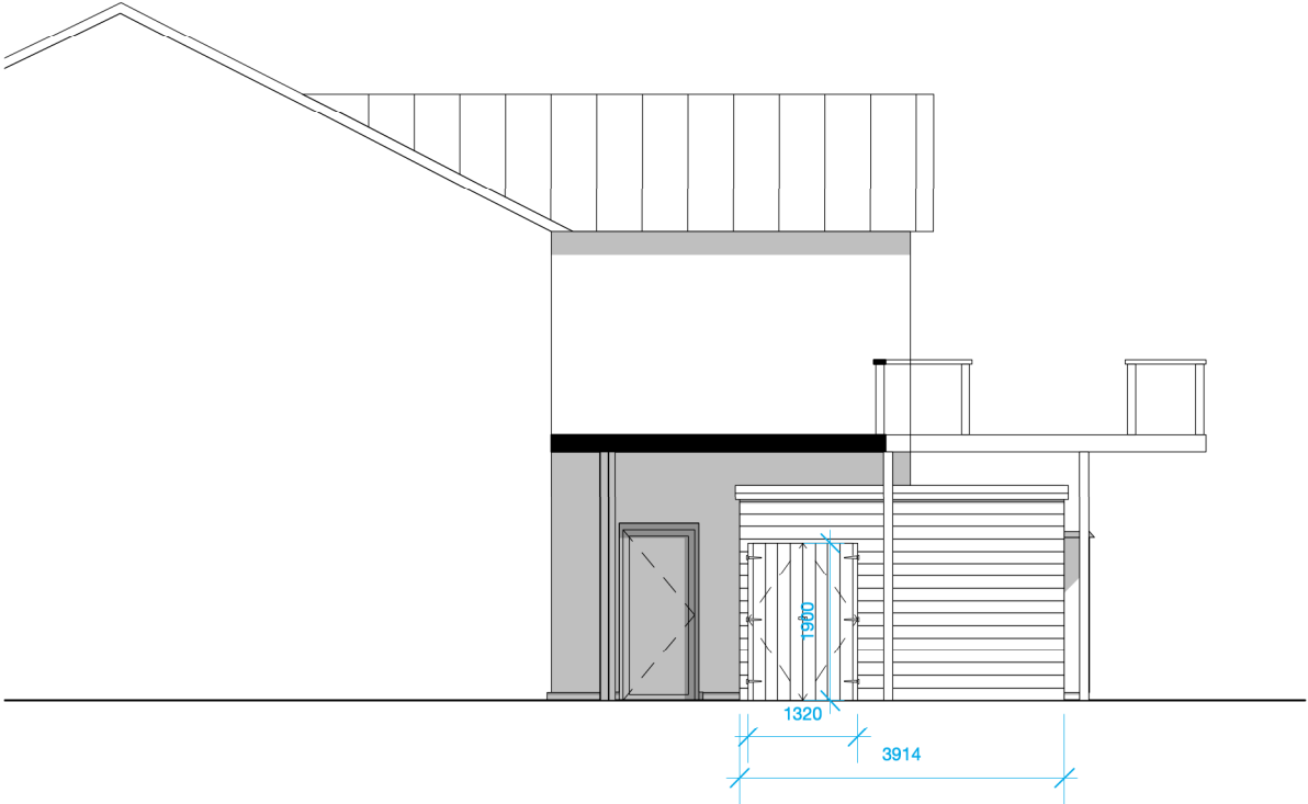
2 Side Elevation 1:100
