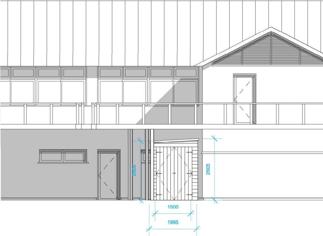
1 Front Elevation 1:100
