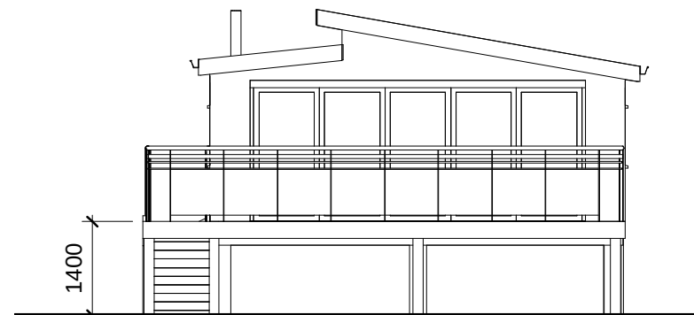
2 North East Elevation 1 : 100
