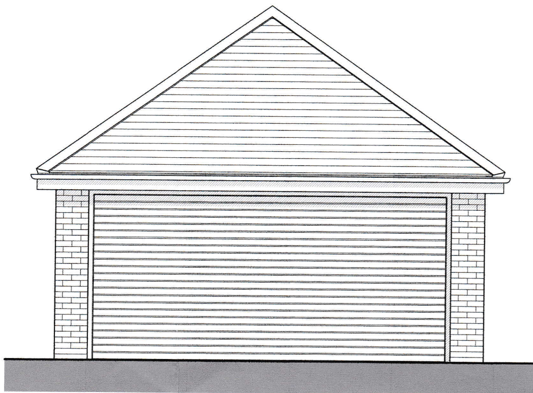
East elevation 1:50
