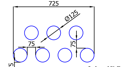
LV DUCT ARRANGEMENT
