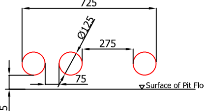
HV DUCT ARRANGEMENT
