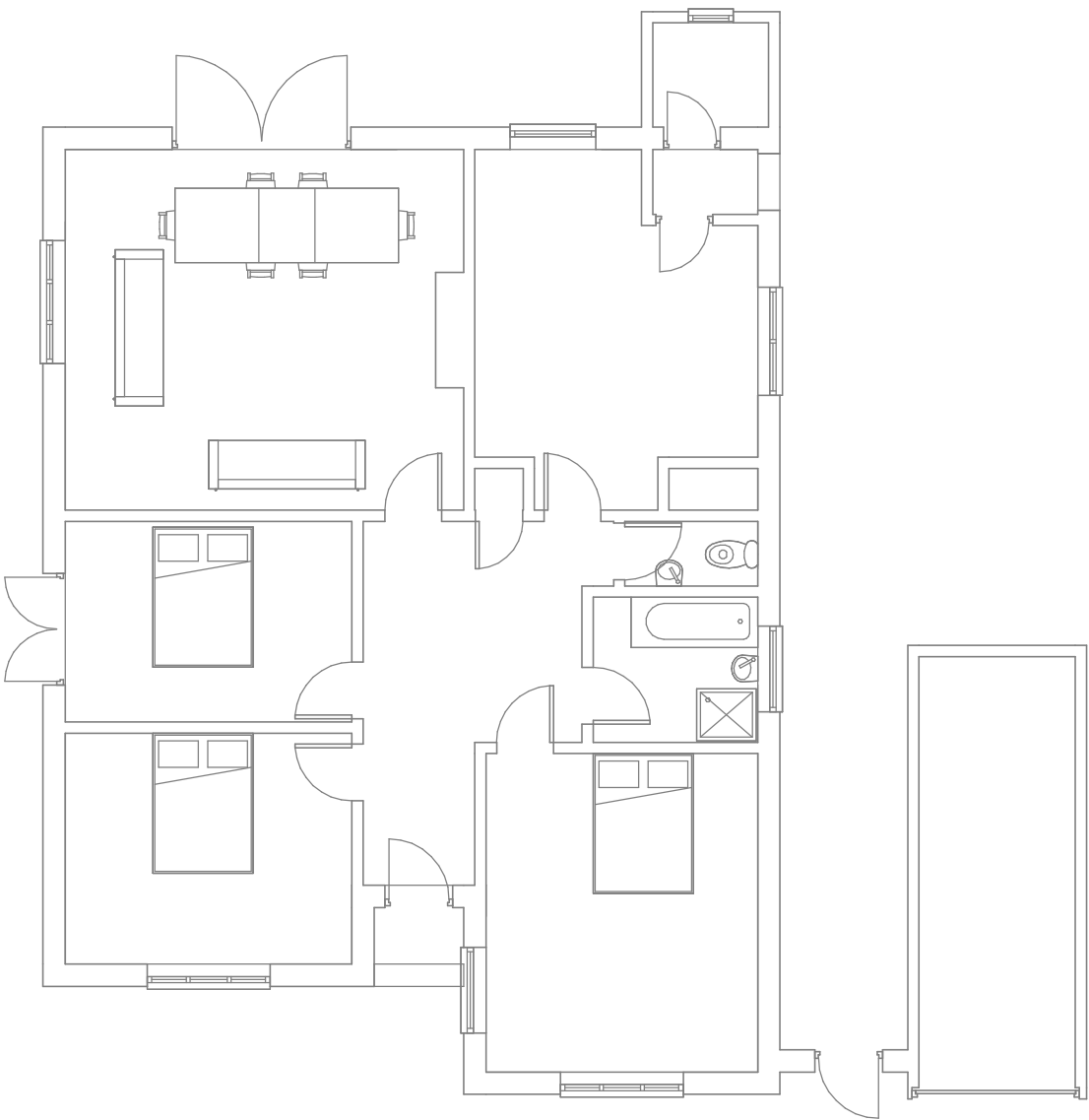
1 Ground Existing 1 : 100
