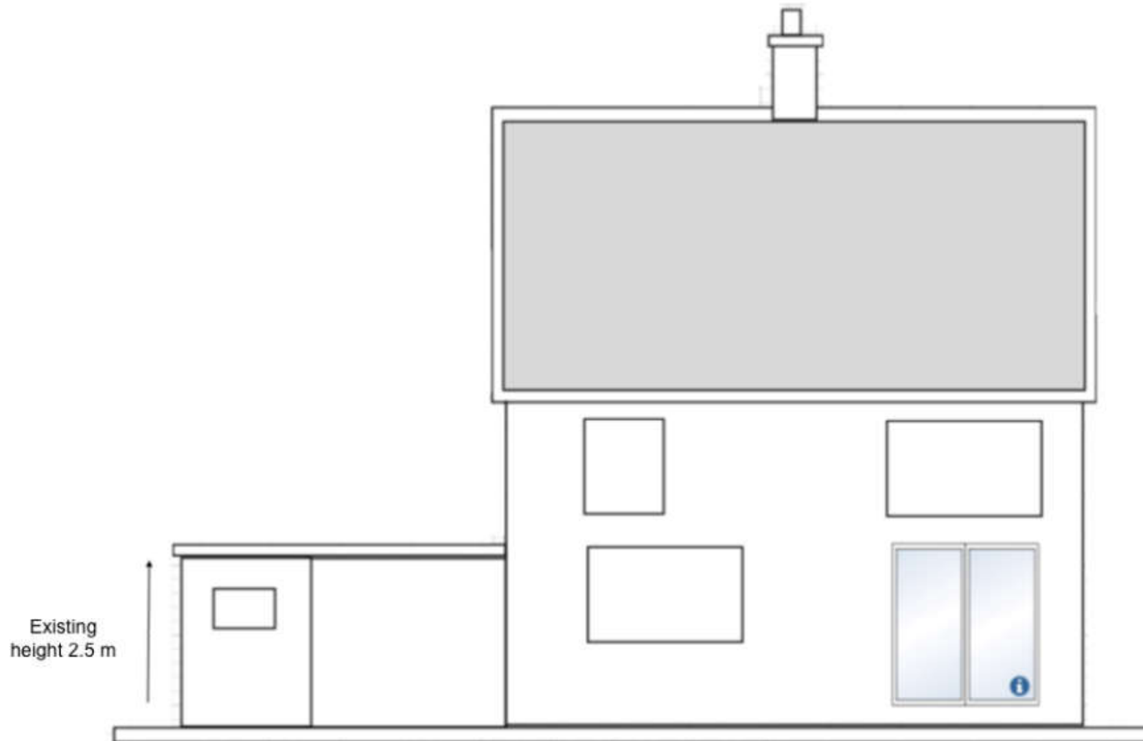
Existing Rear Elevation Scale 1 : 100
