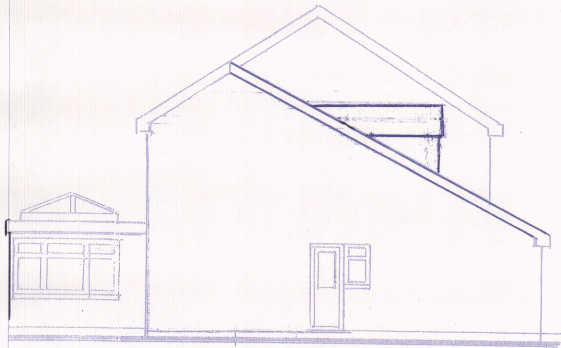
SIDE (NORTH)
