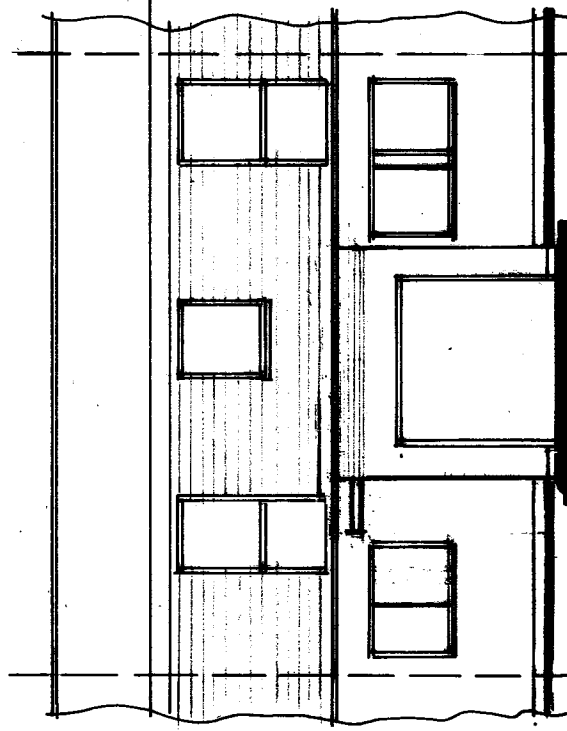
Proposed North West Elevation.
