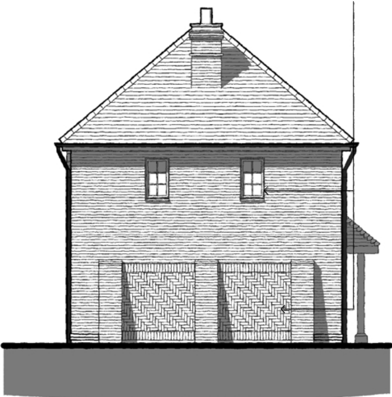
SIDE ELEVATION [2] - 1:100
