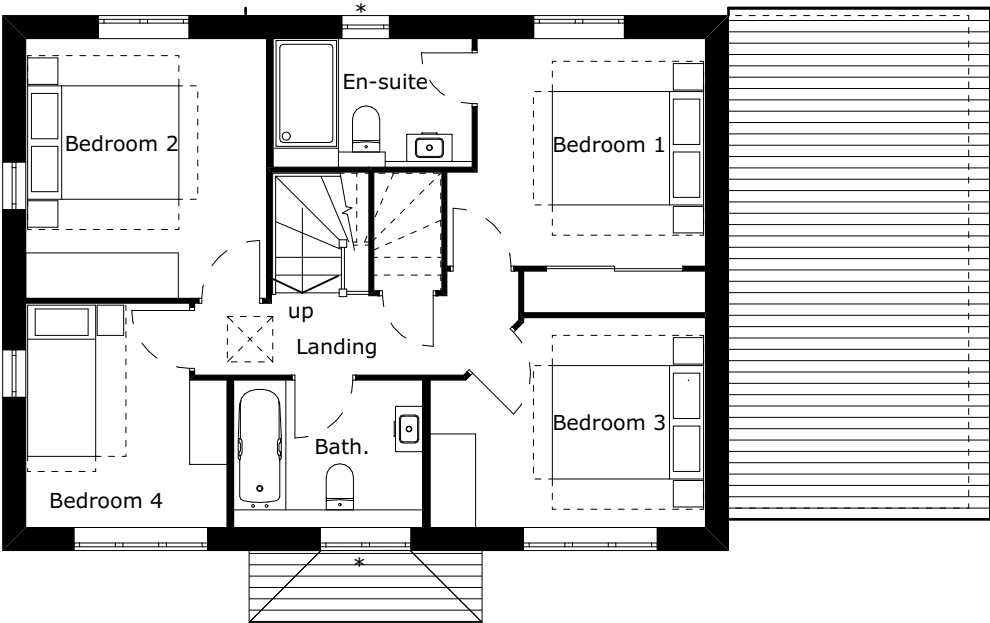
FIRST FLOOR - 1:100
