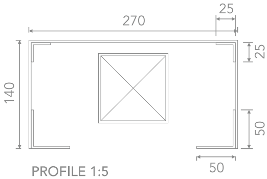
PROFILE 1:5
