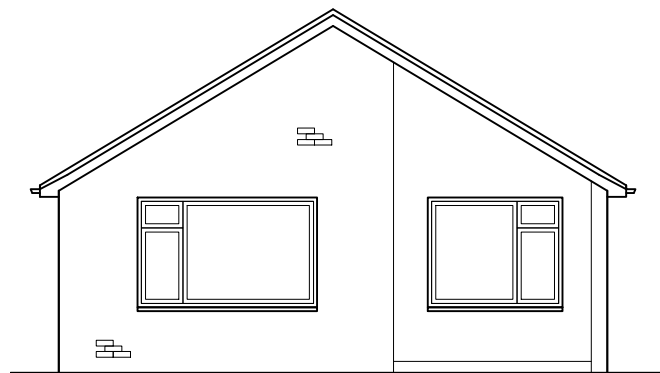
FRONT (N) 1:100
