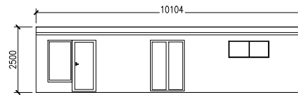
Existing front Elevation
