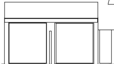
Front elevation (east facing)
