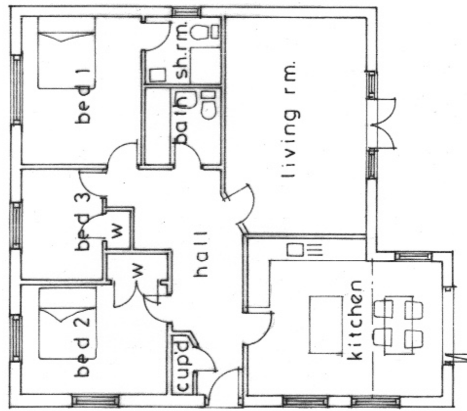
FLOOR PLAN 1:100
