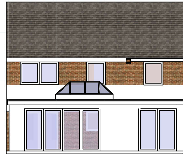
PROPOSED SOUTH ELEVATION
