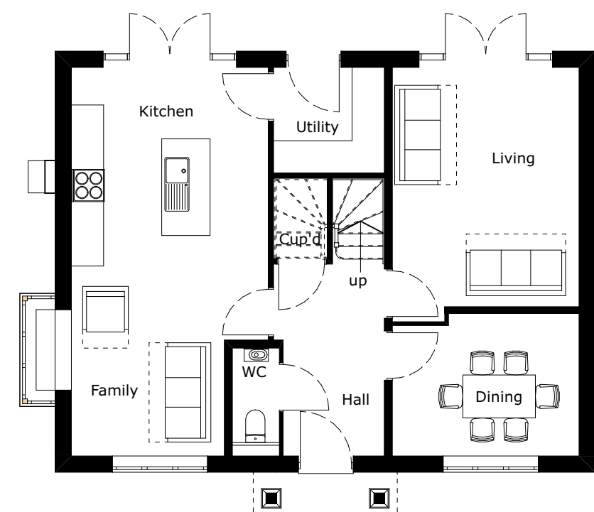
GROUND FLOOR - 1:100
