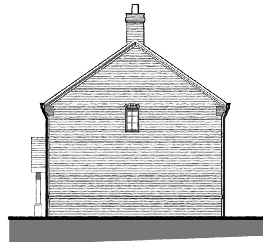
SIDE ELEVATION [2] - 1:100
