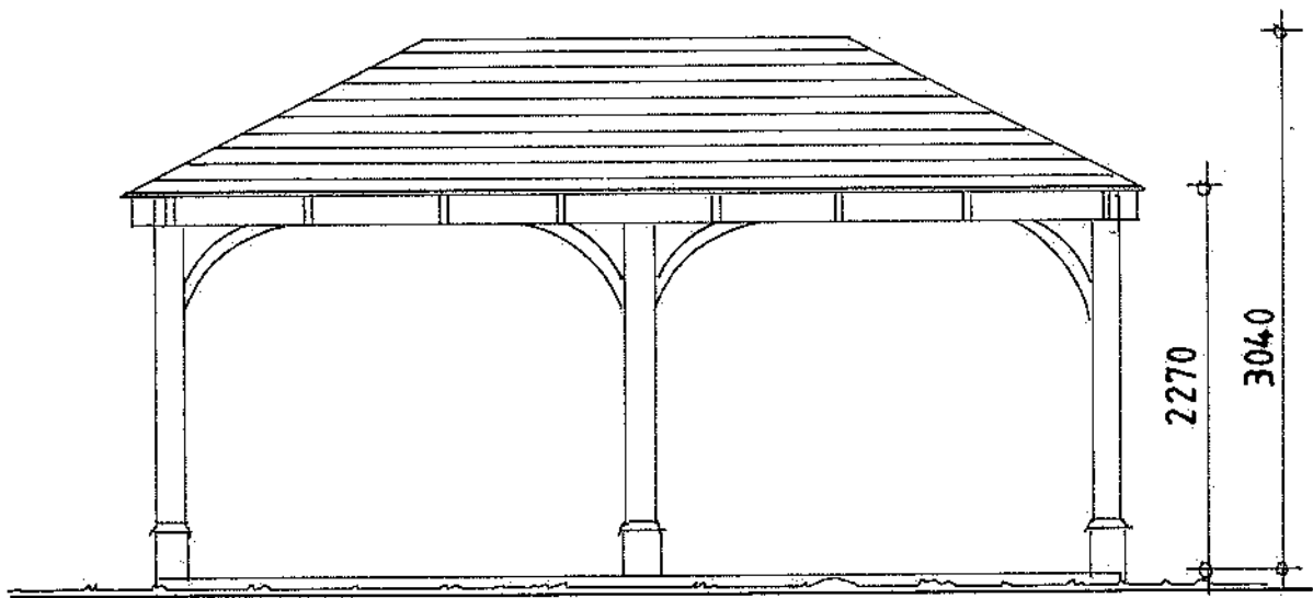
FRONT & REAR
