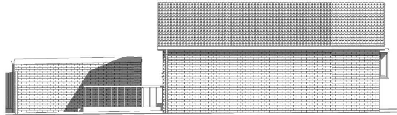
NORTH ELEVATION 1 : 100
