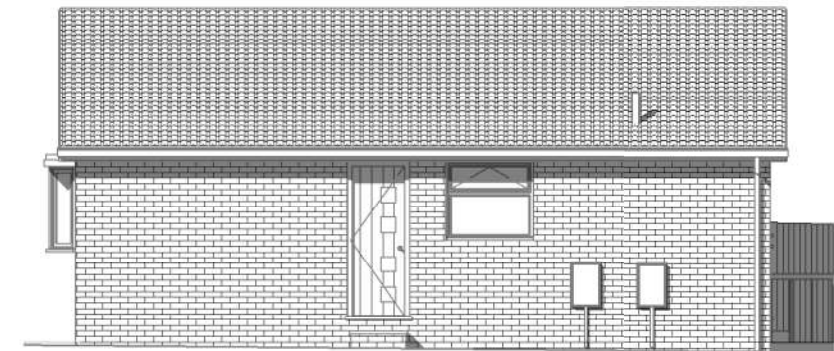
SOUTH ELEVATION 1 : 100
