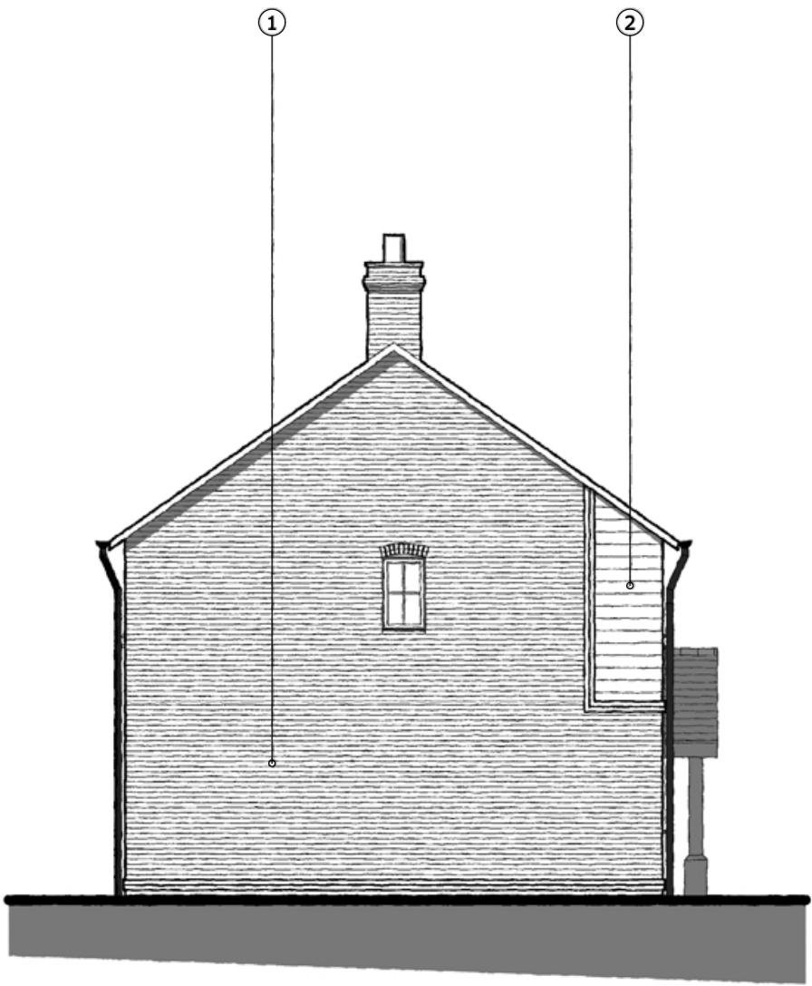
SIDE ELEVATION [1] - 1:100
