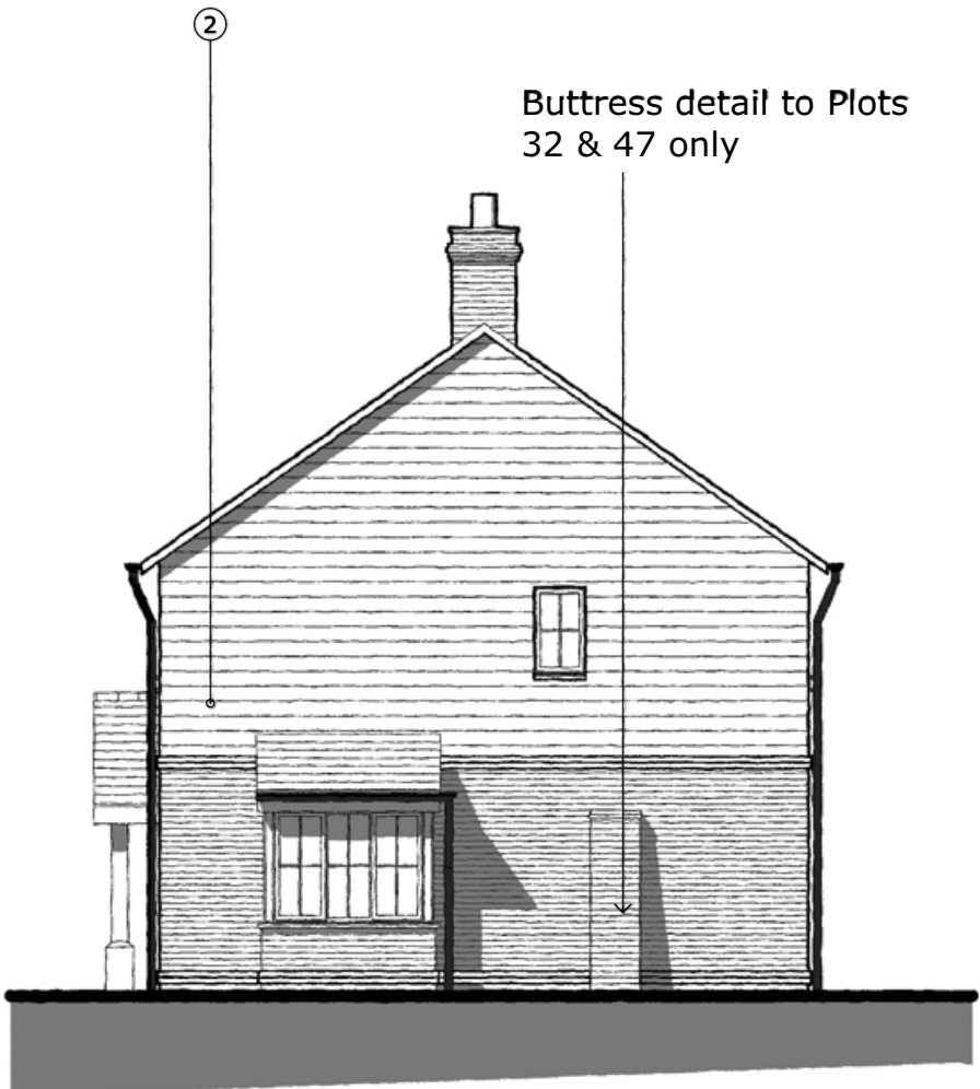
SIDE ELEVATION [2] - 1:100
