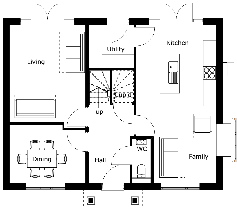
GROUND FLOOR - 1:100
