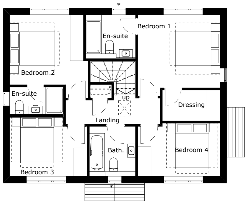
FIRST FLOOR - 1:100
