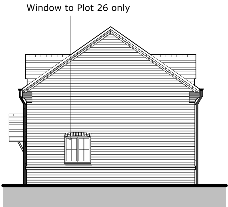
SIDE ELEVATION [2] - 1:100
