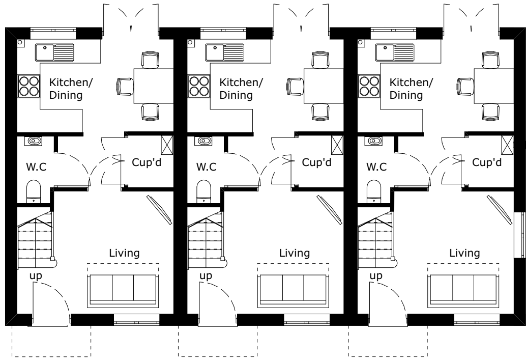
GROUND FLOOR - 1:100
