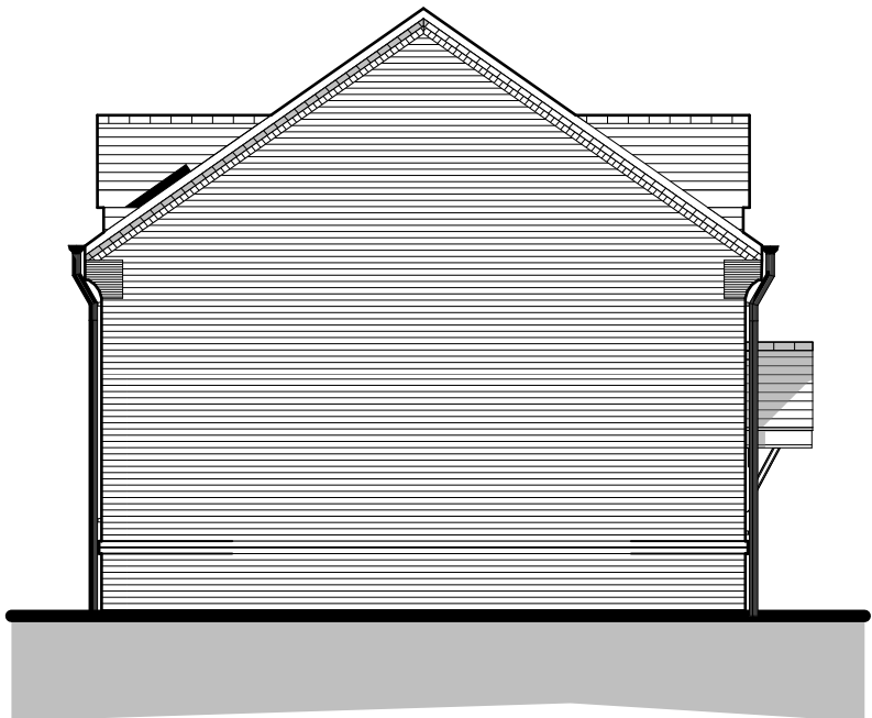
SIDE ELEVATION [1] - 1:100
