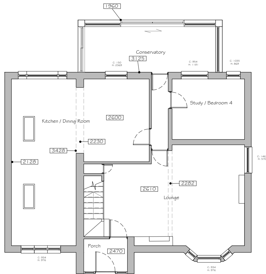
Existed Ground Floor Plan Scale 1:100
