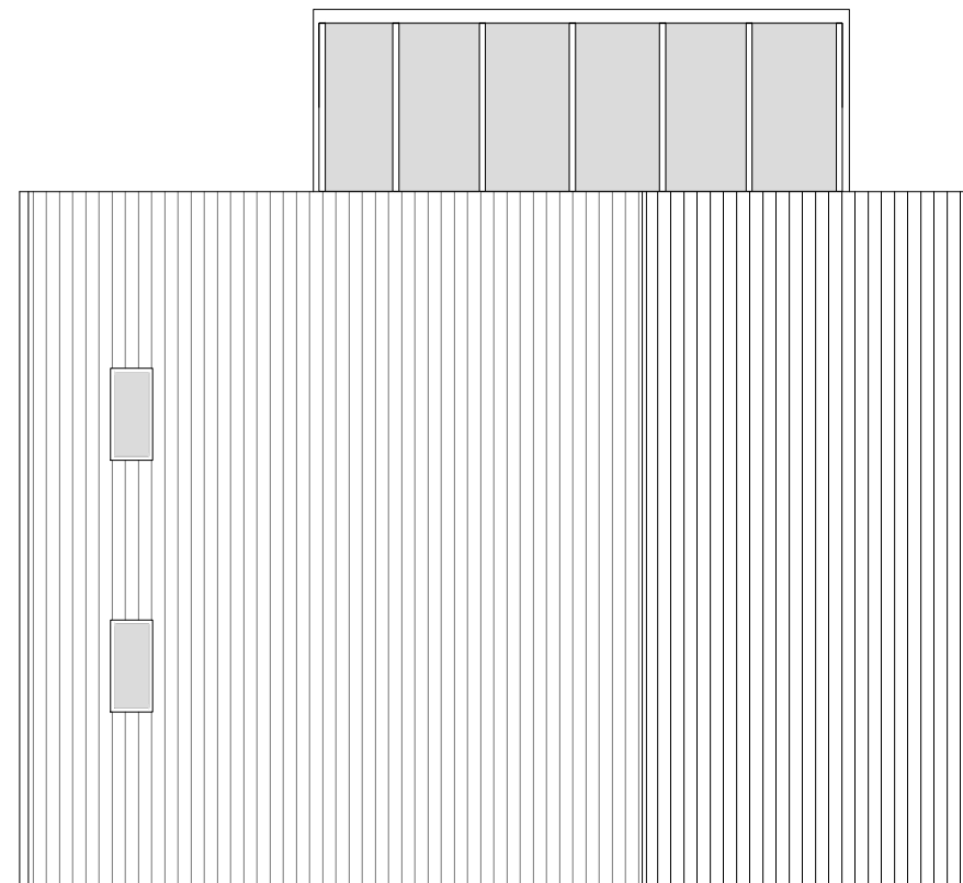
Existed Roof Plan Scale 1:100
