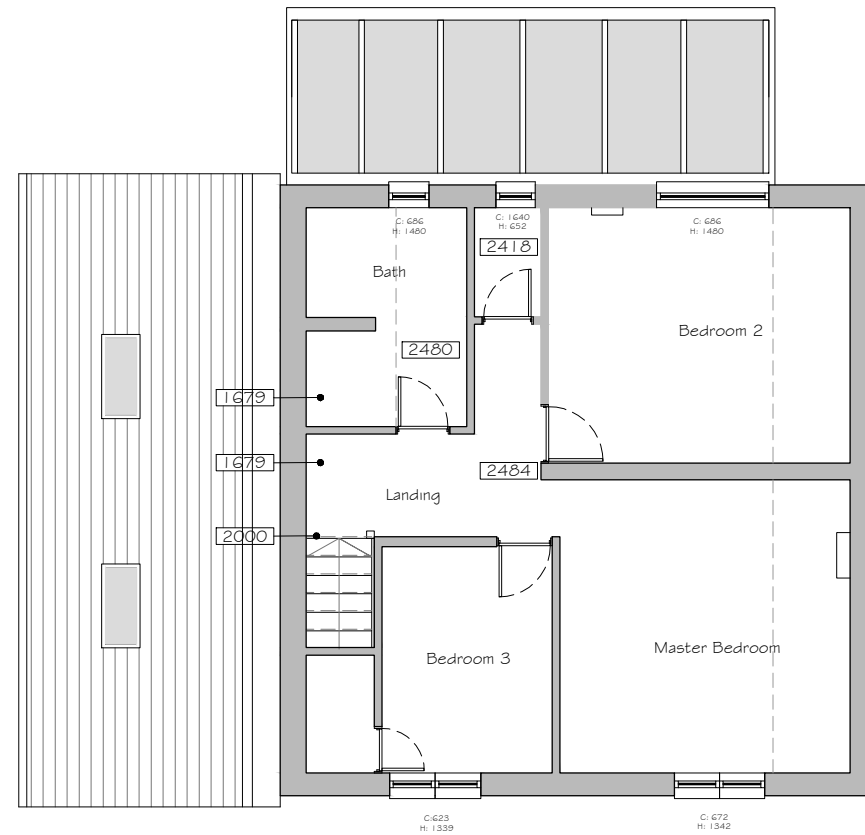
Existed First Floor Plan Scale 1:100
