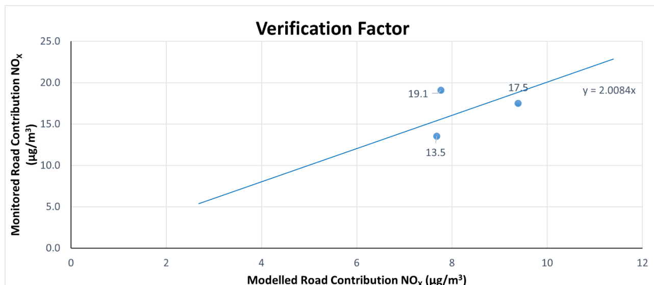
Figure E1 - Comparison of Measured Road-NO x with Unadjusted Modelled Road-NO x
