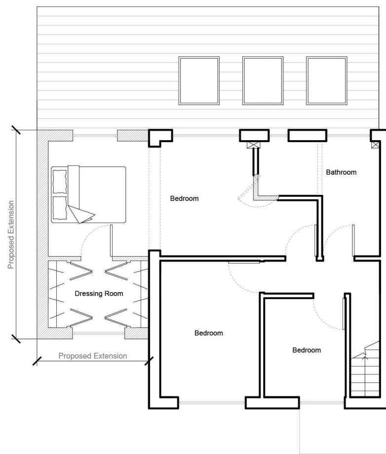
Proposed First Floor Plan scale A3 1:100
