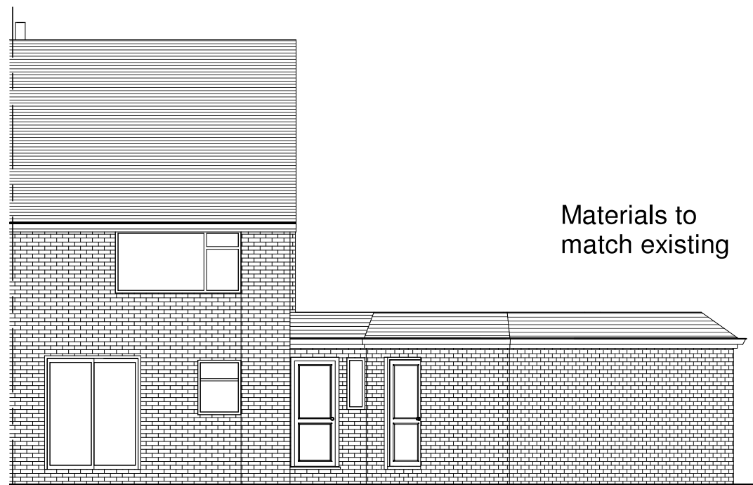
Proposed SE Elevation
