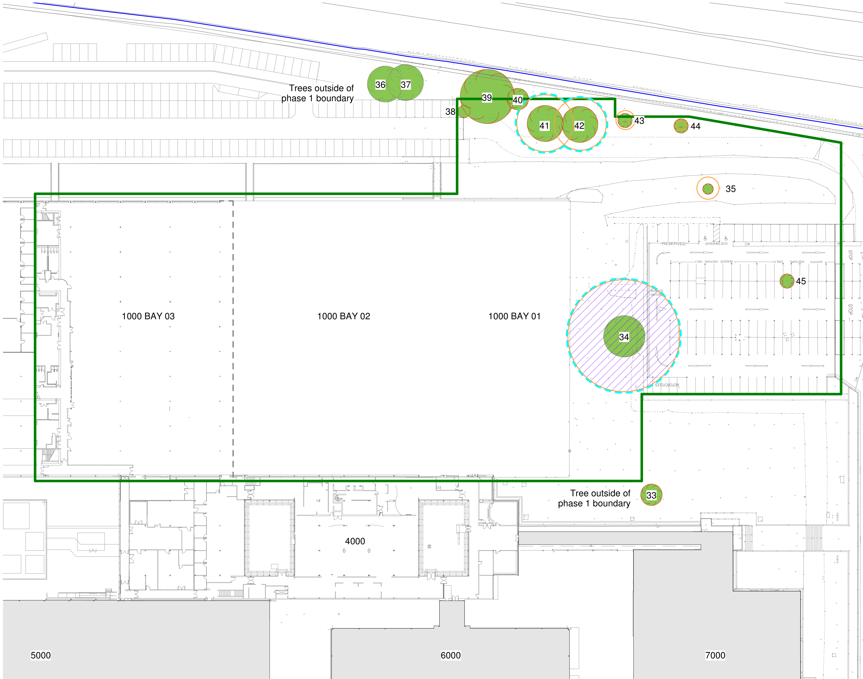
Phase 1 Works with Tree Protection Plan 1 : 500
