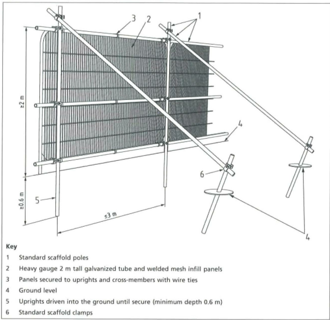
Example of appropriate protective barrier fence
