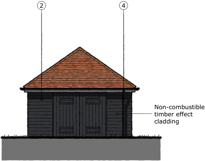
FRONT ELEVATION - 1:100
