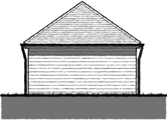
SIDE ELEVATION [2] - 1:100
