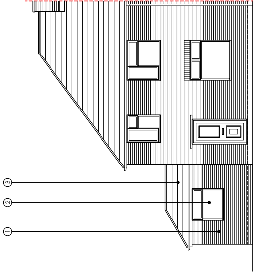
PROPOSED NORTH WEST ELEVATION SCALE 1:100
