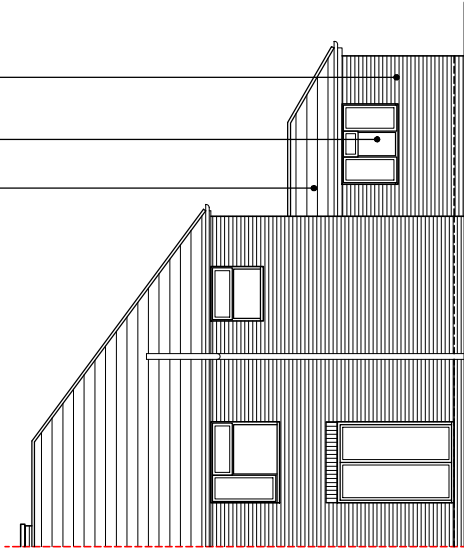
PROPOSED SOUTH EAST ELEVATION SCALE 1:100
