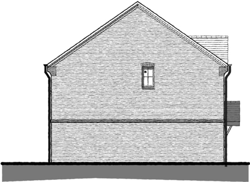
SIDE ELEVATION [1] - 1:100
