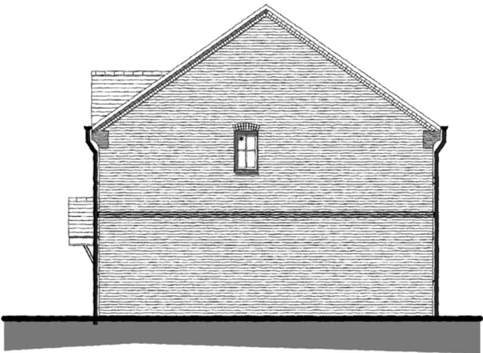
SIDE ELEVATION [2] - 1:100
