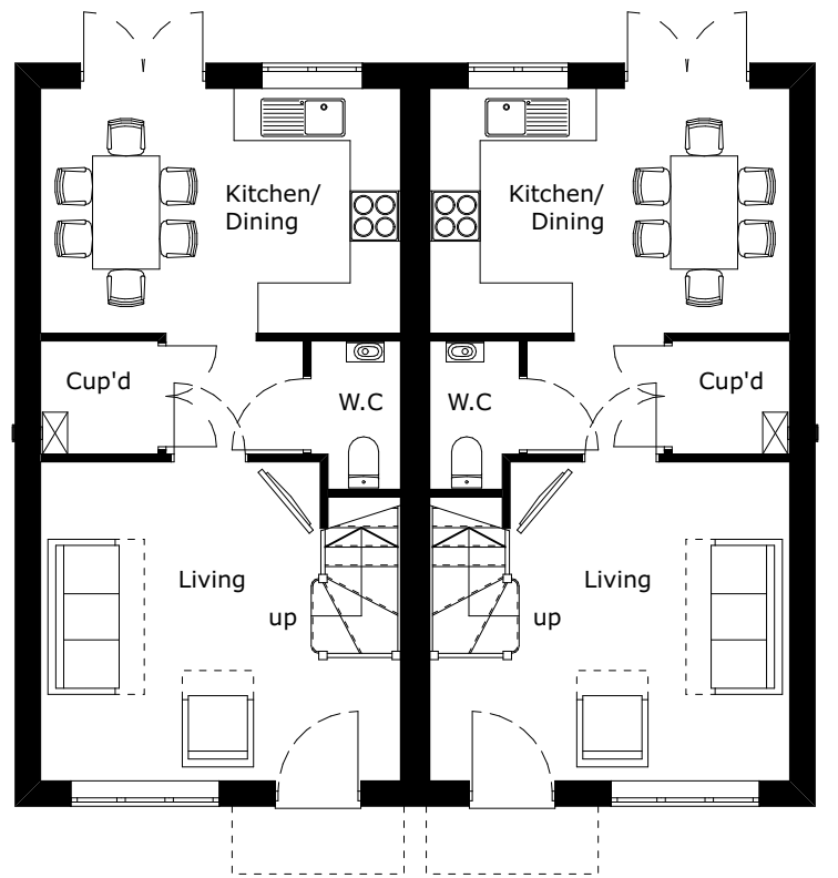
GROUND FLOOR - 1:100
