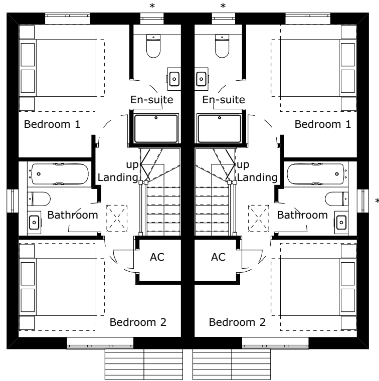
FIRST FLOOR - 1:100
