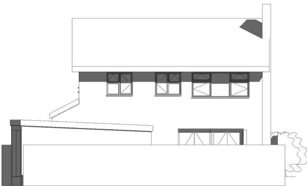
Existing West Elevations
