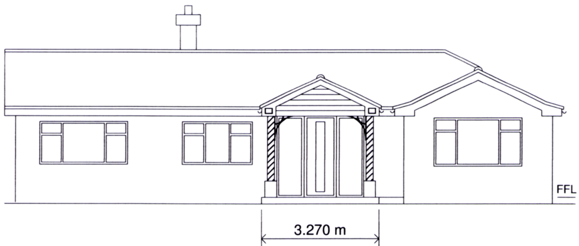
MODIFIED EAST ELEVATION
