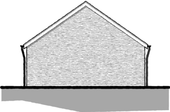
SIDE ELEVATION [1]- 1:100
