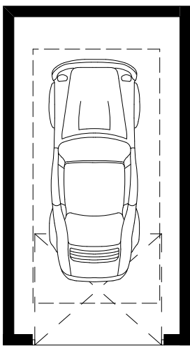
FLOOR PLAN - 1:100
