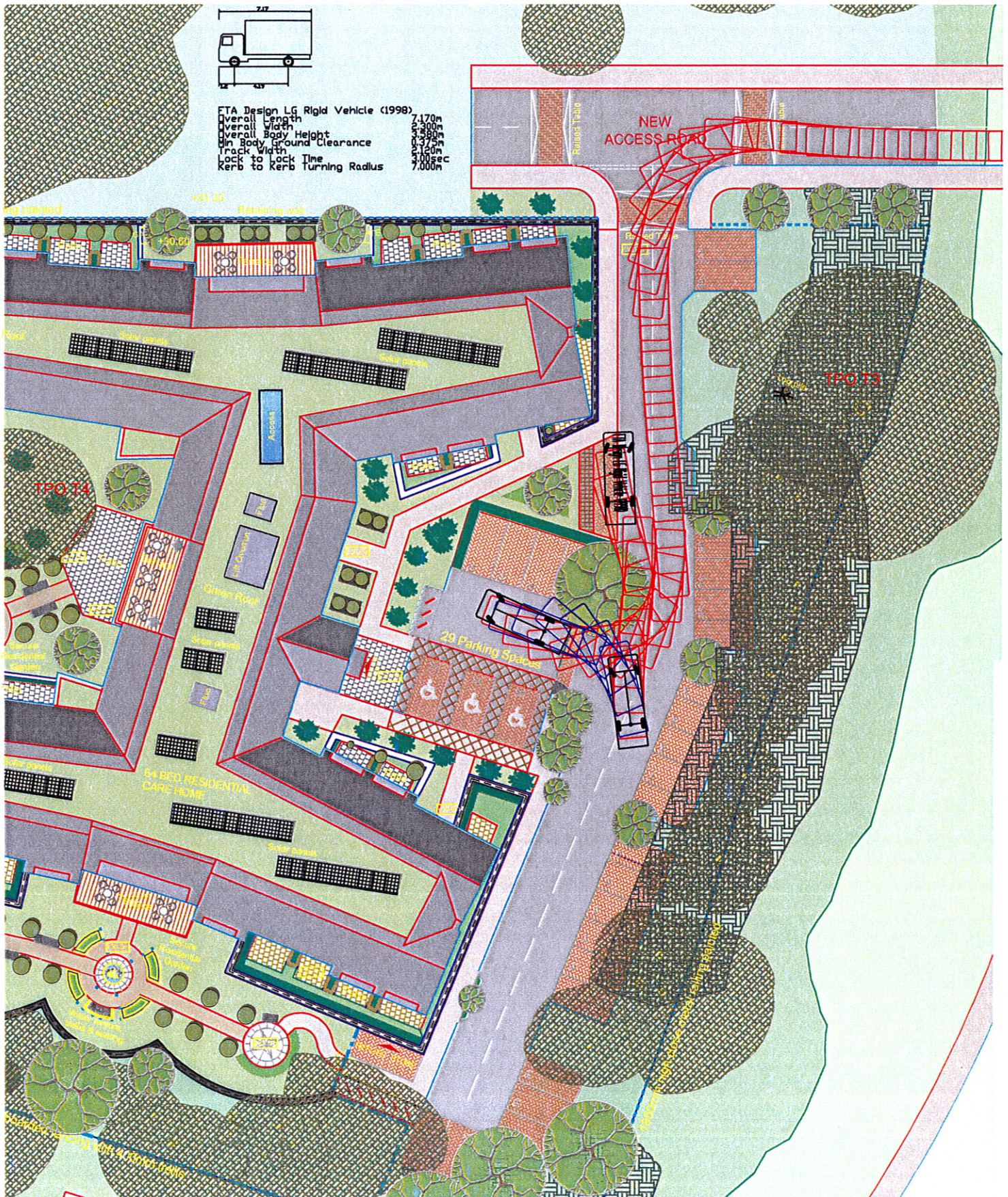
FIGURE 13 Tracking of delivery vehicle within site
