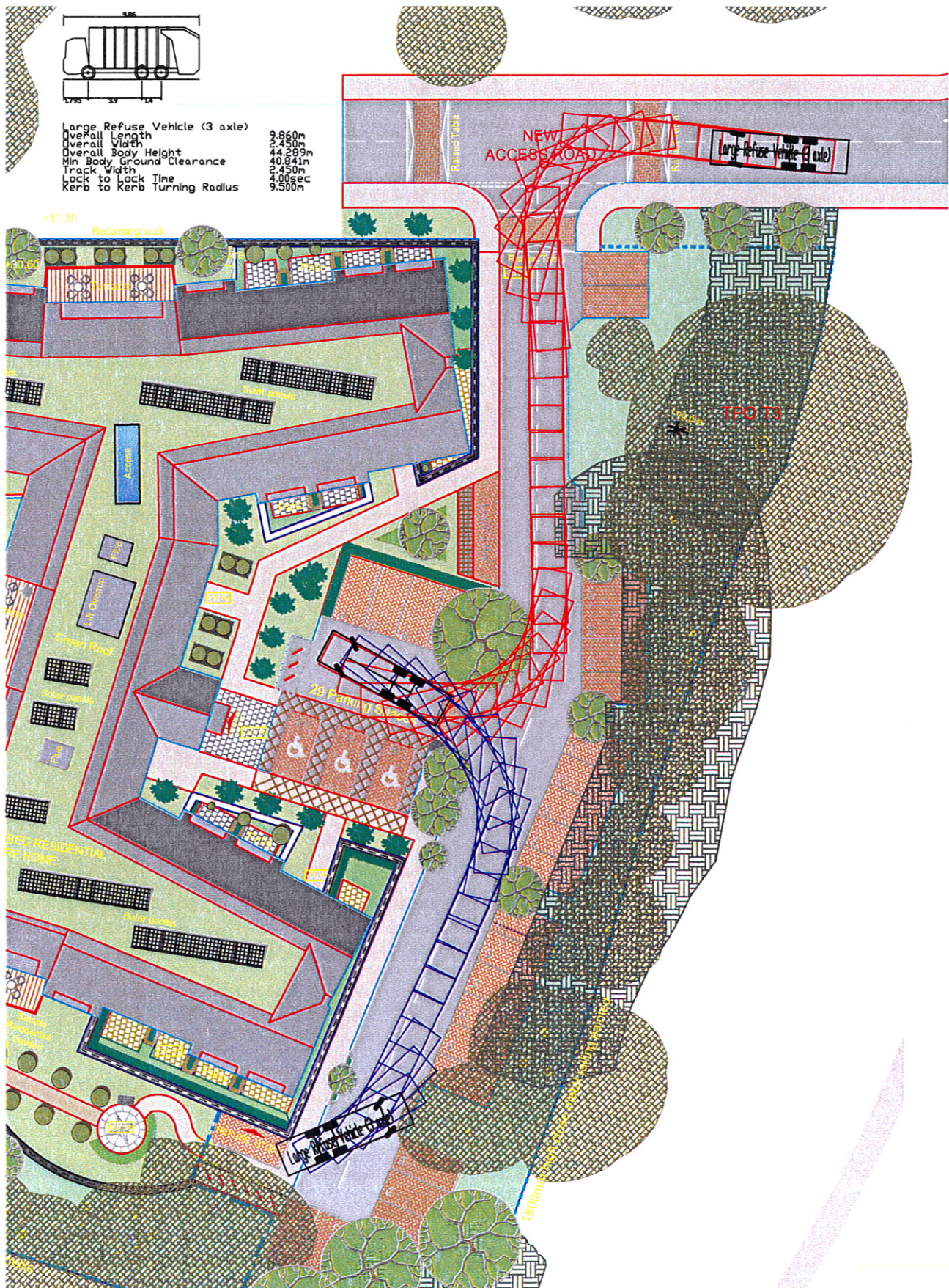
FIGURE 14 Tracking of 3-axle refuse vehicle within site
