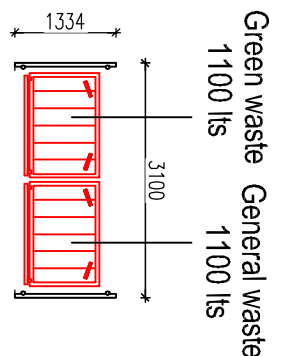
Refuse Store 1 & 2
