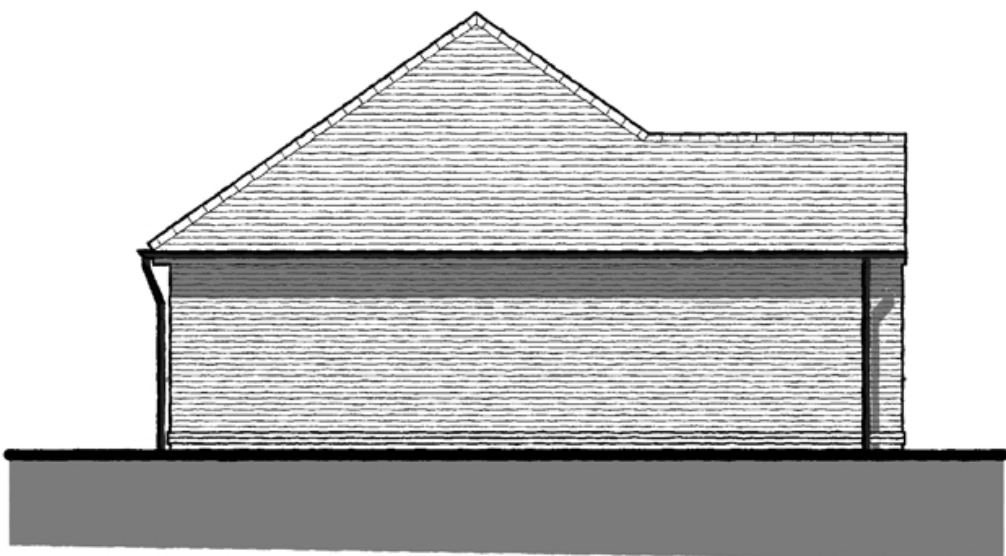
SIDE ELEVATION [1] - 1:100
